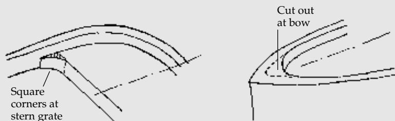
FIG. 4 – Carving the Deck
